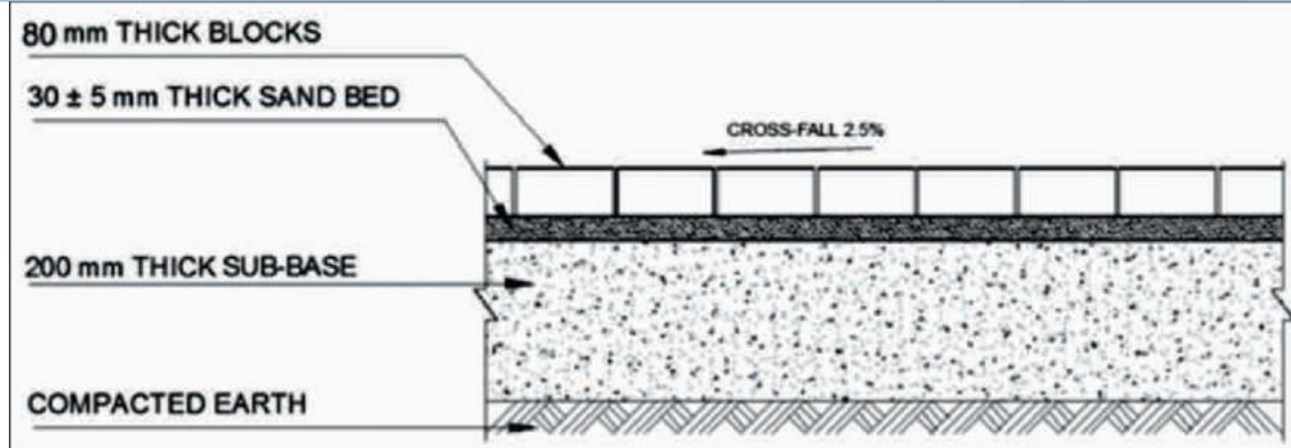
Figure 2- 5: Typical Cross-Section for Footpaths (R3)
