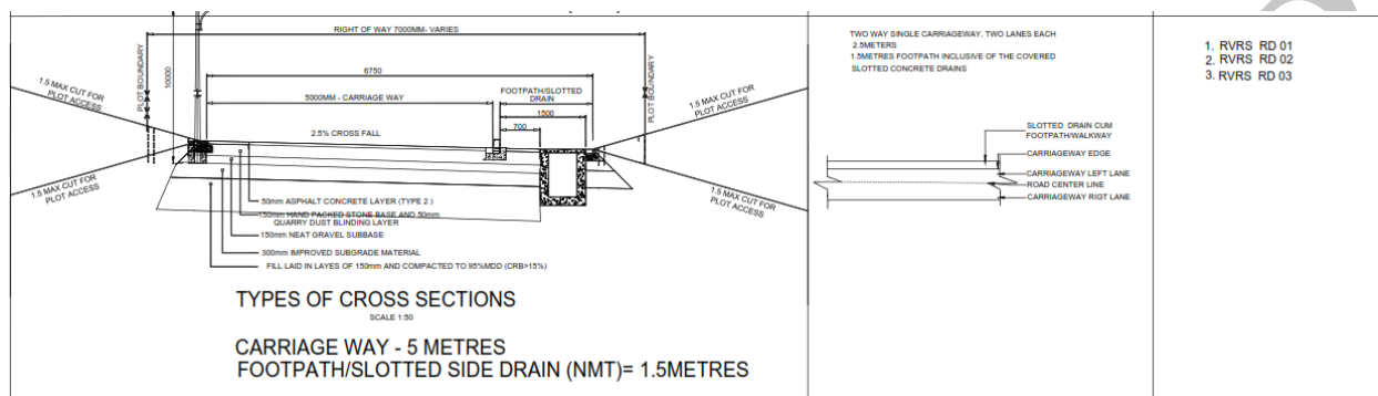
Figure 4 - Typical Road Cross Sections – Bosnia/Riverside Settlement
