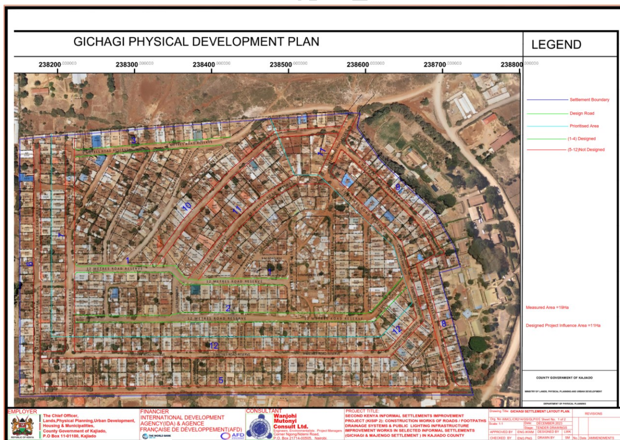
Figure 8 - Layout plan of the Gichagi Settlement, Ngong Town
